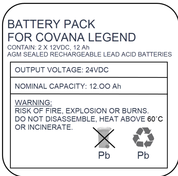
FIGURE 14: BATTERY SPECIFICATION LABEL
