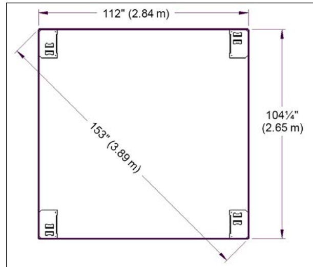
FIGURE 15: FOUNDATION DIAGONAL
